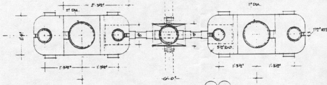
PLAN SECTION — (D D) —
